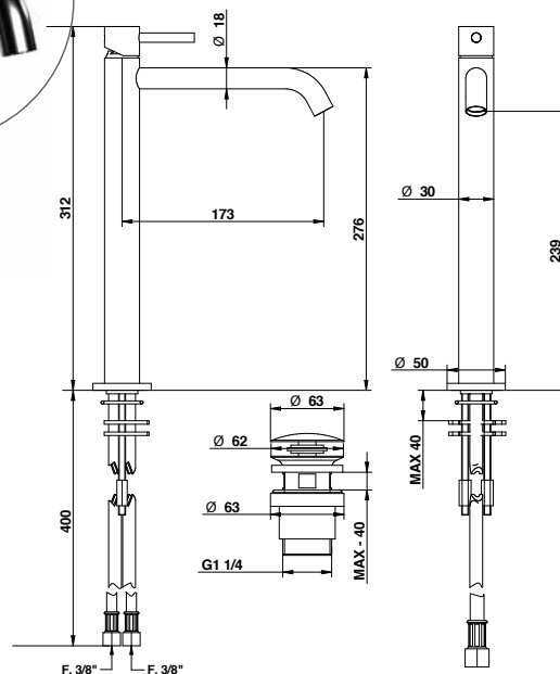
Miscelatore lavabo alto con piletta clic-clac High basin mixer with clic-clac waste
