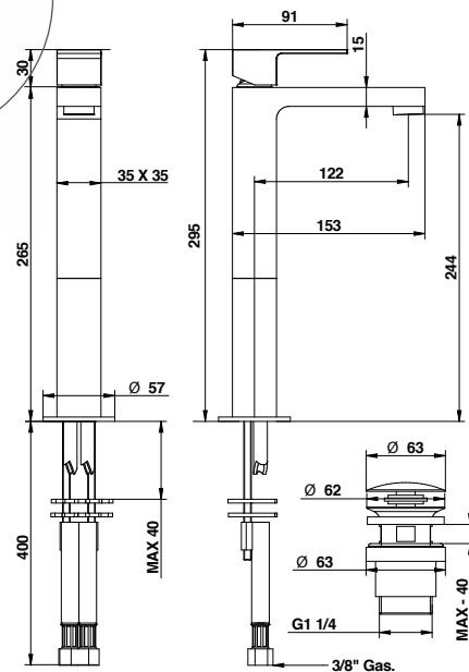
Miscelatore lavabo alto con piletta clic-clac High basin mixer with clic-clac waste
